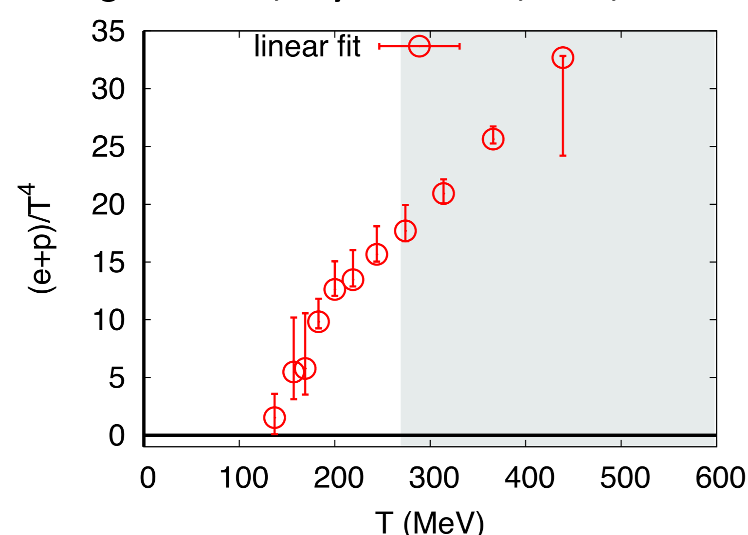
Fig. 4, K. Kanaya et. al., EPJ Web of Conference, 175, 07023, pp.1-8
