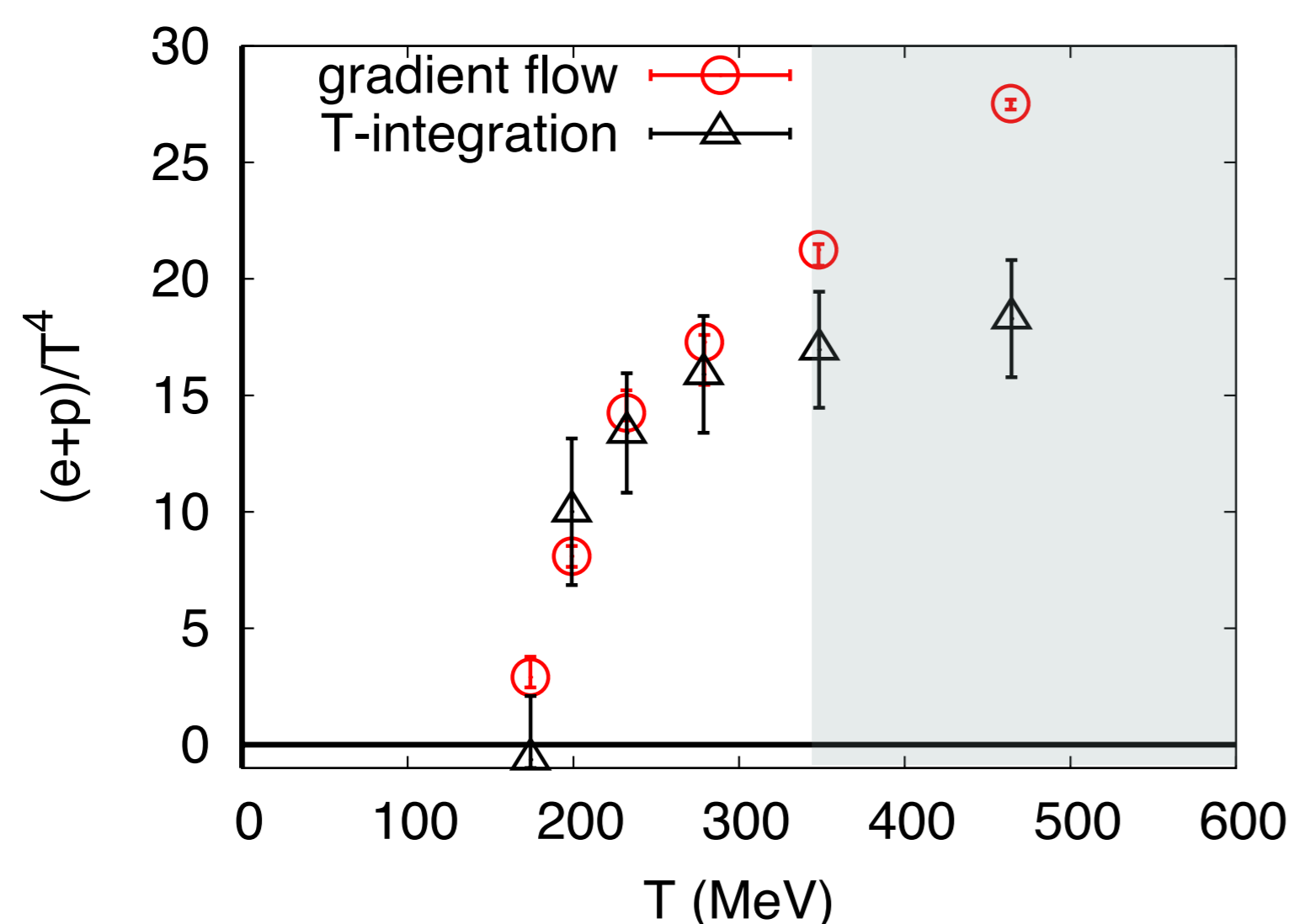
Fig. 3, Y. Taniguchi et. al., Phys. Rev. D 96, no. 1, 014509 (2017)
