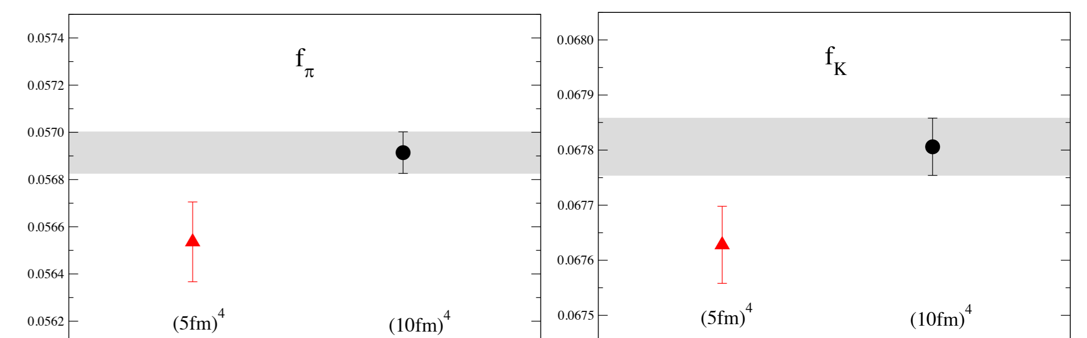
Fig2, K.-I. Ishikawa et. al., https://arxiv.org/abs/1807.06237
