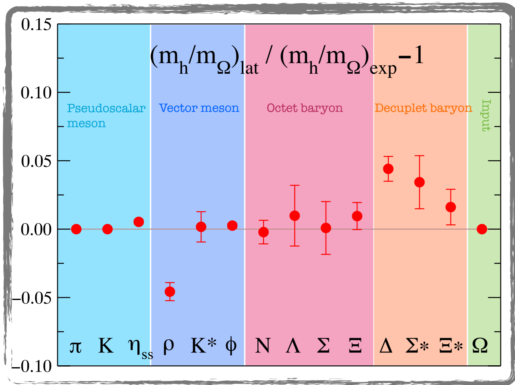
Fig1, K.-I. Ishikawa et. al., https://arxiv.org/abs/1511.09222
