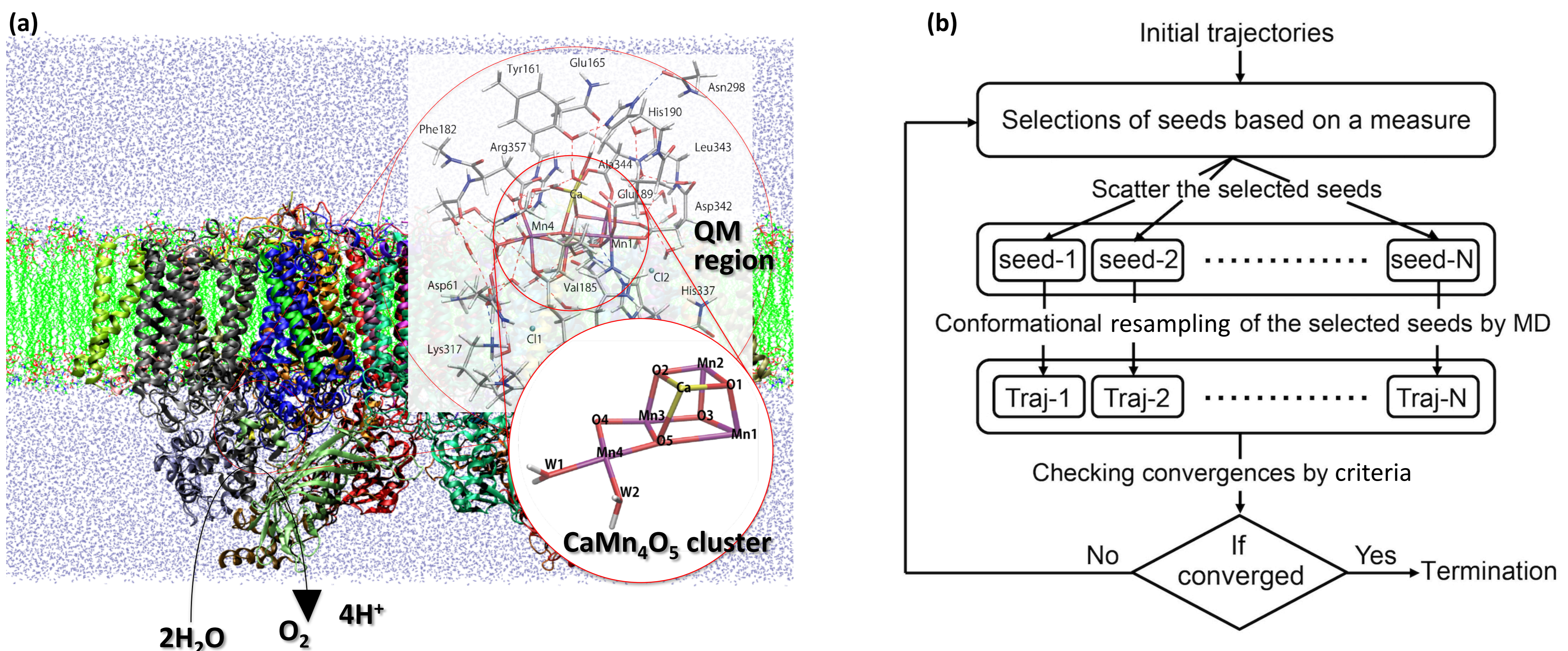
Fig. 1: (a) QM/MM model of oxygen evolving complex in photosystem II. Key intermediate states in the catalytic reaction “ 2\text{H}_2\text{O} + 4h\nu \rightarrow 4\text{H}^+ + 4\text{e}^- + \text{O}_2 ” have been investigated using the large model. [M. Shoji et al., Catal. Soc. Technol., 3, 1831 (2013).]
