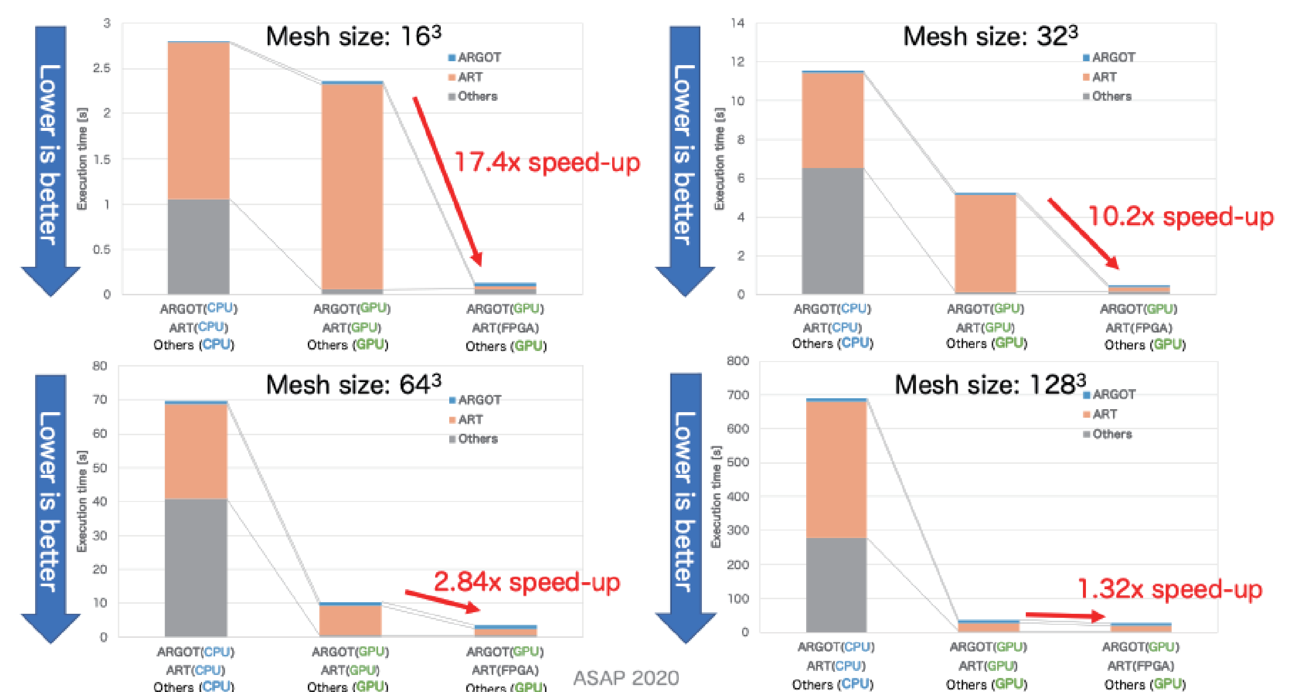
GPU+FPGA co-computation performance in early-universe object-formation simulation
