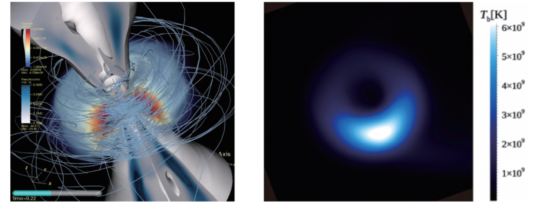
Fig.1 Left: Black hole accretion disks and jets in general relativistic radiative magnetohydrodynamic simulations Right: Black hole shadow reproduced by general relativistic radiative transfer calculations
